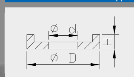
Valve Stopper Compression Base Valve dimensions
